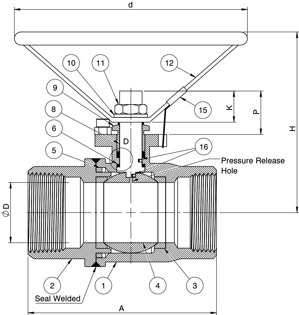
PRESSURE RATING 2000 WOG
