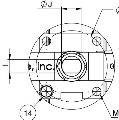
Actuator ISO Mounting Flange 5211
