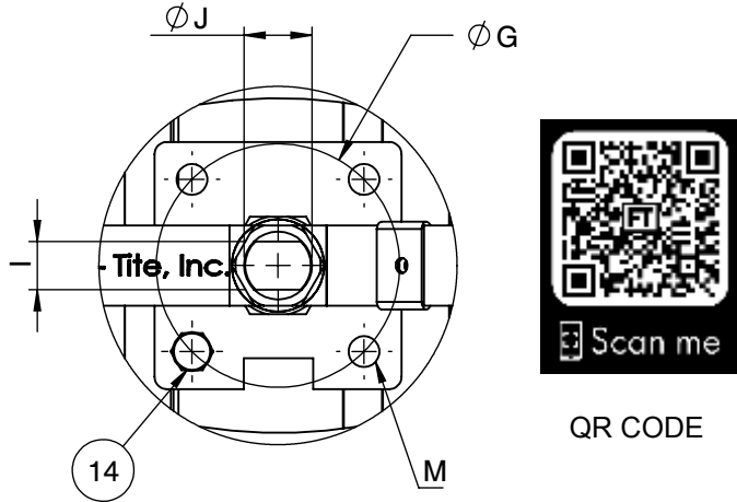
Actuator ISO Mounting Flange 5211
