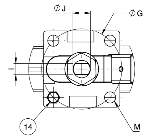
Actuator ISO Mounting Flange 5211
