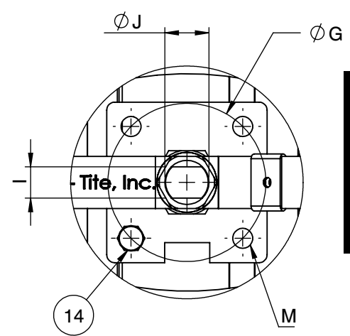
Actuator ISO Mounting Flange 5211
