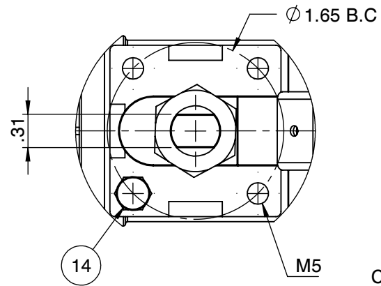
Actuator ISO Mounting Flange (F05)
