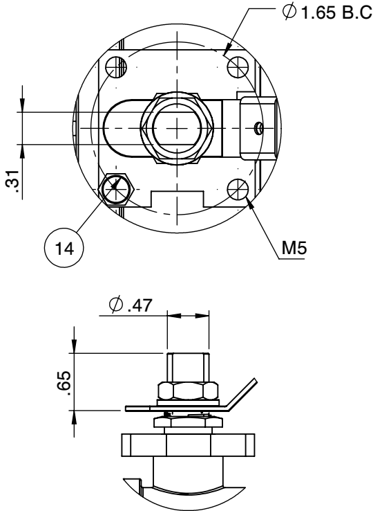
Actuator ISO Mounting Flange (F05)
