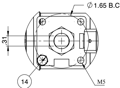
Actuator ISO Mounting Flange (F05)
