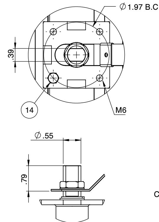
Actuator ISO Mounting Flange (F07)
