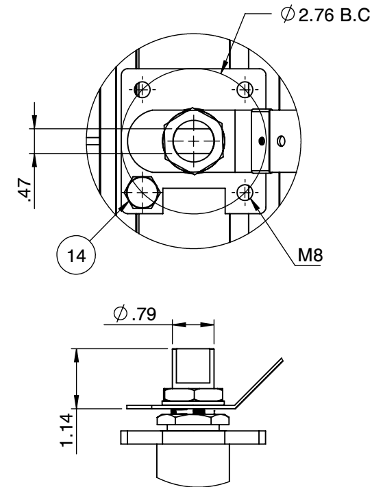
Actuator ISO Mounting Flange (F10)
