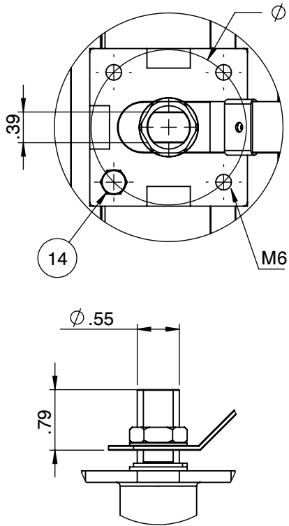
Actuator ISO Mounting Flange (F07)
