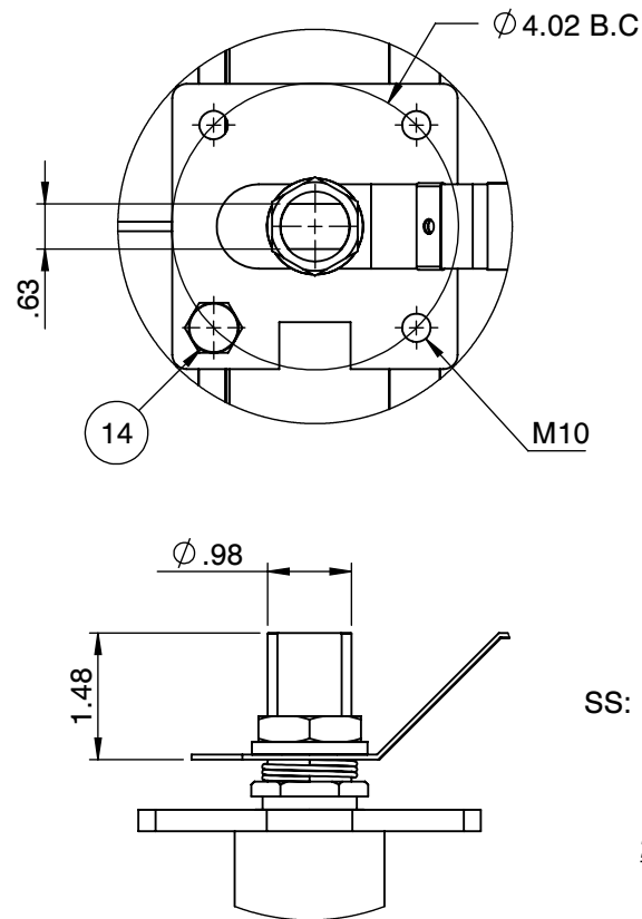
Actuator ISO Mounting Flange (F12)
