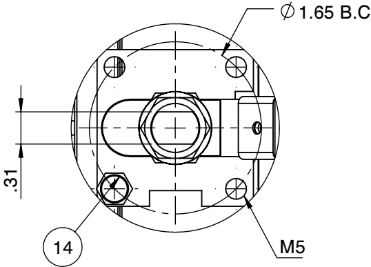
Actuator ISO Mounting Flange (F05)
