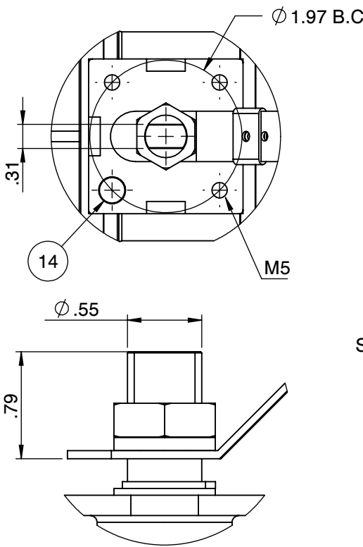
Actuator ISO Mounting Flange (F07)
