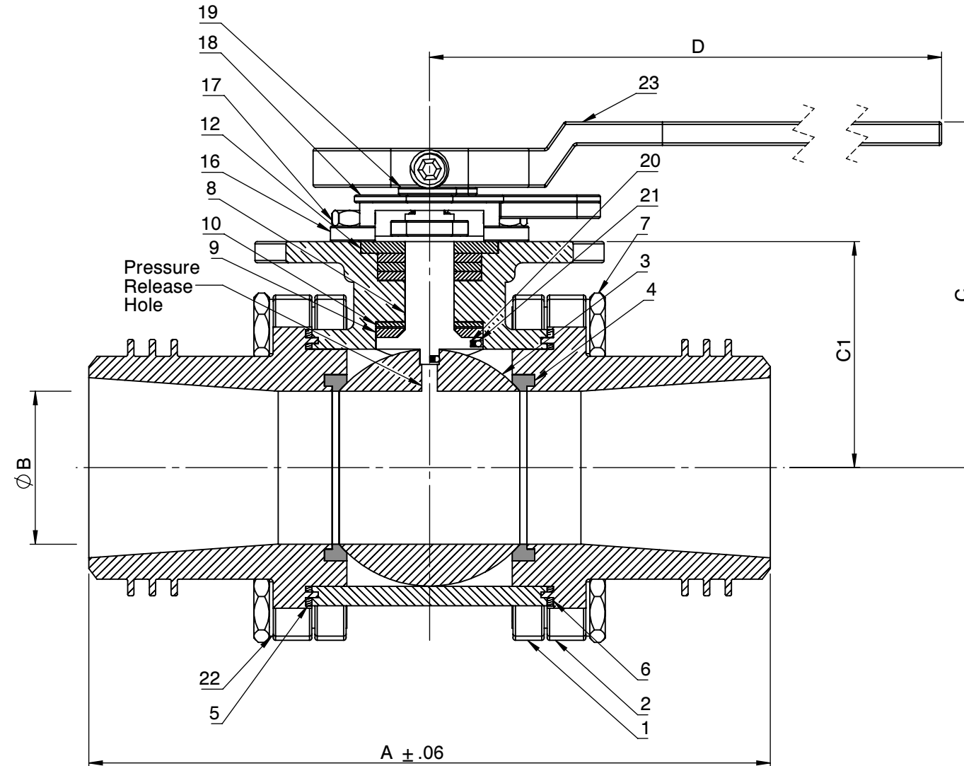
ANSI PRESSURE RATING CLASS 600/2250 WOG
