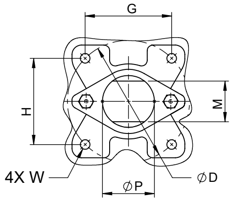
Actuator ISO Mounting Flange (F16)
