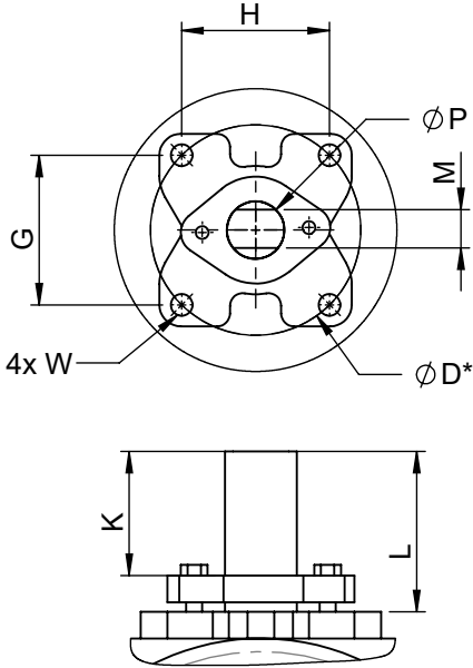
Actuator ISO Mounting Flange (F12)
