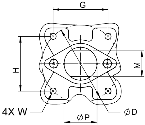
Actuator ISO Mounting Flange (F12)
