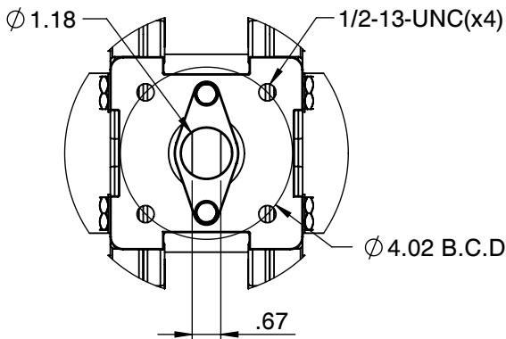
Actuator ISO Mounting Flange (F10)
