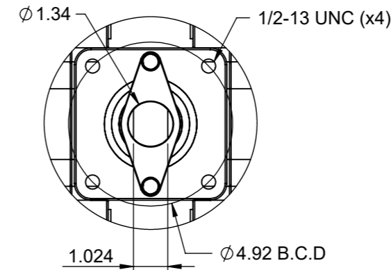
Actuator ISO Mounting Flange (F12)
