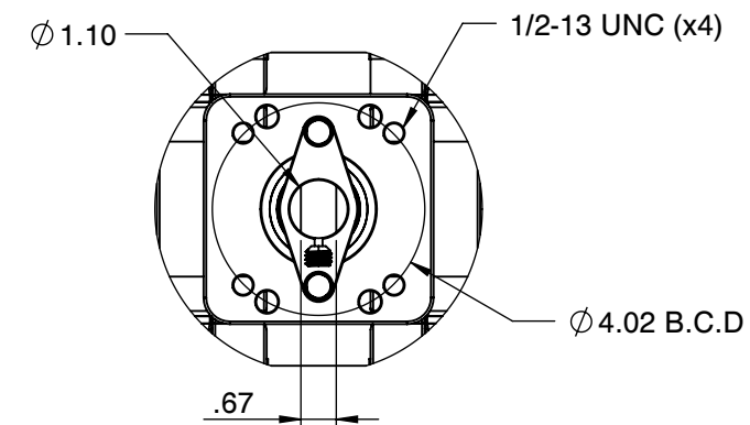
Actuator ISO Mounting Flange (F10)
