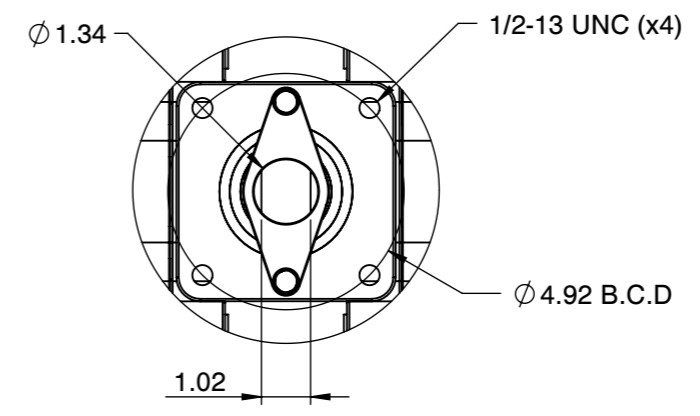
Actuator ISO Mounting Flange (F12)
