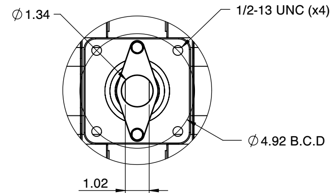
Actuator ISO Mounting Flange (F12)
