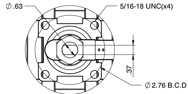
Actuator ISO Mounting Flange (F07)
