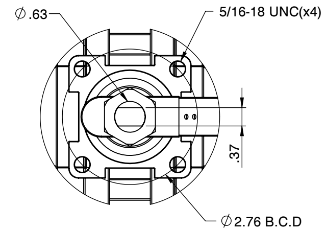
Actuator ISO Mounting Flange (F07)
