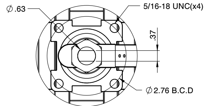
Actuator ISO Mounting Flange (F07)
