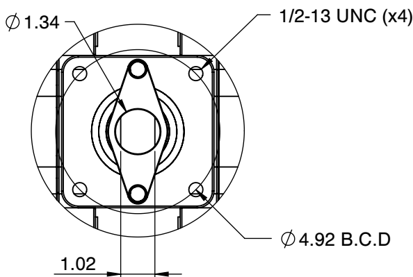
Actuator ISO Mounting Flange (F12)
