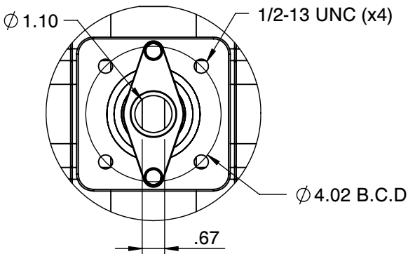
Actuator ISO Mounting Flange (F10)
