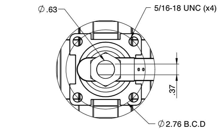
Actuator ISO Mounting Flange (F07)
