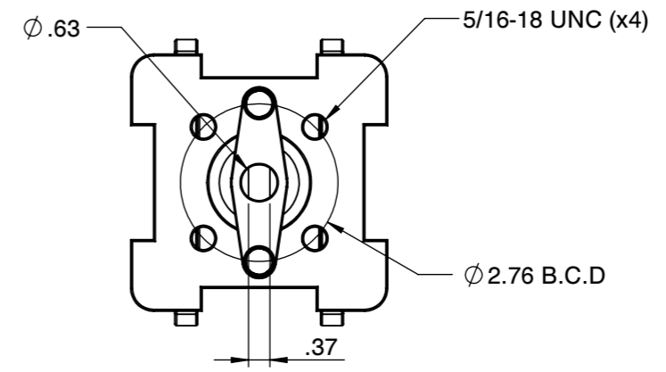
Actuator ISO Mounting Flange (F07)
