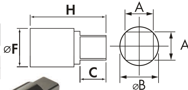
Custom Fabricated Stem Extensions
