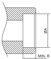
SOCKET END AS PER B16.11
