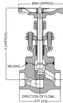
WELDED DESIGN
