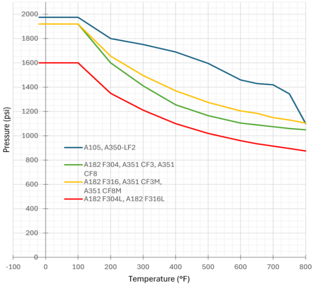
Class 800 Pressure-Temperature Ratings
