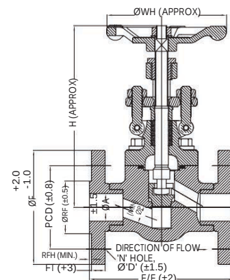
FLANGE END DESIGN
