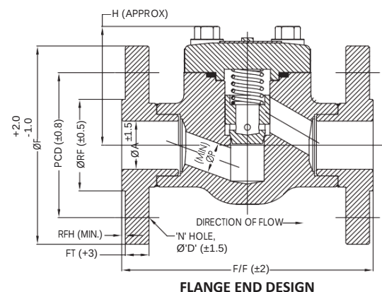
FLANGE END DESIGN
