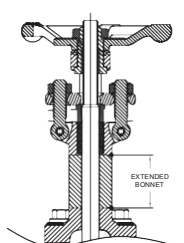
Extended Bonnet
