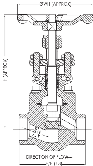
BOLTED DESIGN
