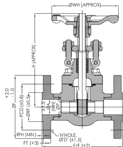
FLANGE END DESIGN
