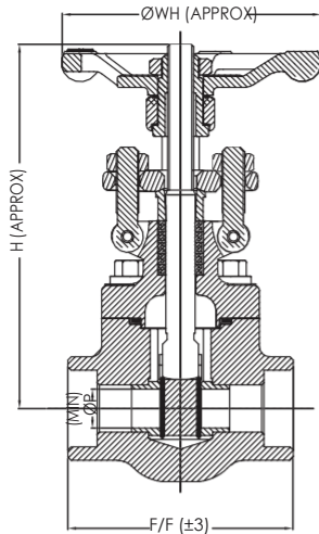
BOLTED DESIGN
