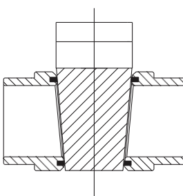
Inserted PTFE
