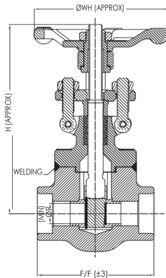
WELDED DESIGN
