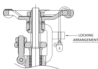
Locking Arrangement
