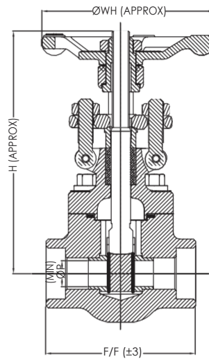
BOLTED DESIGN
