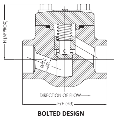
BOLTED DESIGN
