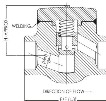
WELDED DESIGN
